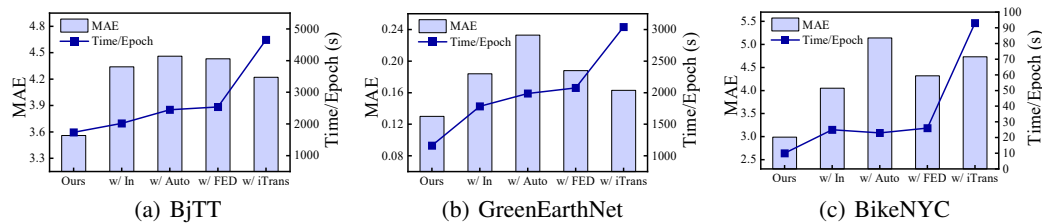
Figure 7: E 2 -CSTP with Transformer-based variants across datasets.
