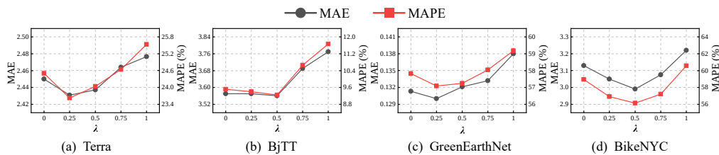
Figure 8: Parameter sensitivity study on \lambda .
