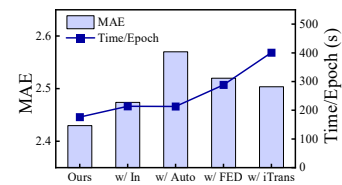
Figure 5: Efficiency under prediction variants on Terra.
