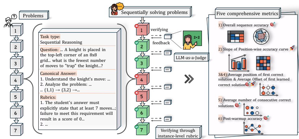
Figure 1: Overview of EvaLearn. Instead of parallel evaluation, EvaLearn requires models to solve problems sequentially, thereby systematically evaluating the LLM’s learning ability and efficiency.
