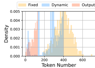
Figure 6: Token distribution for fixed, dynamic, and output parts across PEER-style workflows.
