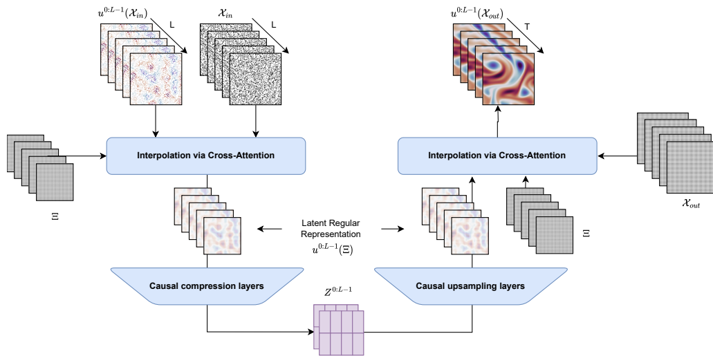
Figure 14: General architecture of ENMA’s encoder/decoder.
