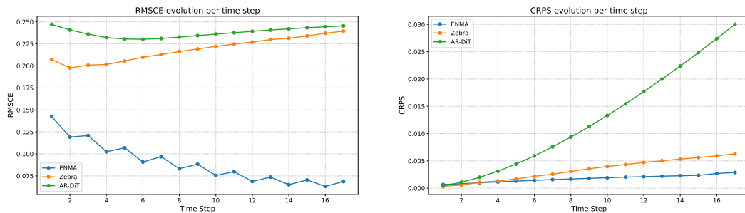
(a) RMSCE evolution over time. Lower values indicate better uncertainty calibration.
