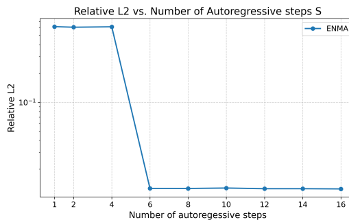
Figure 25: Relative L2 error as a function of the number of autoregressive steps S . Performance improves markedly around S = 6 and plateaus thereafter.
