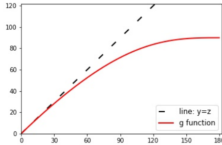
Figure 5: Curve of the function g(\theta) . As can be seen, g(\theta) is monotonic, and is approximately the identity function y = \theta in the small angle region ( \theta \ll 90^\circ ).
