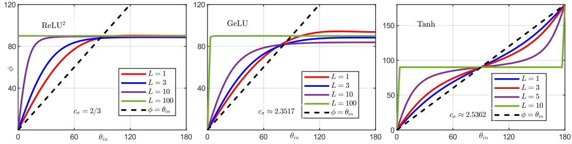
Figure 2: Better separation for non-ReLU activation functions. Left: \text{ReLU}^2 , Middle: GeLU, Right: tanh. All plots are model gradient angle \phi vs. input \theta_{in} .
