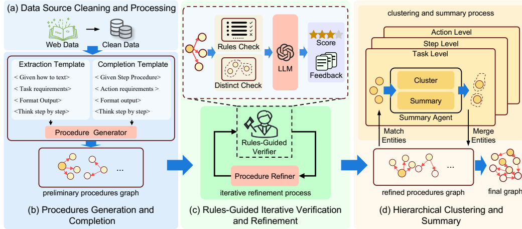
Figure 3: Overview of our automatic construction pipeline: (a) Data source cleaning and processing. (b) A Generator extracts steps with attributes from the data source and performs actions completion. (c) A Verifier and A Refiner iteratively validate procedures against designed rules while progressively refining them. (d) A Summary Agent hierarchically clusters and merges redundant procedures.
