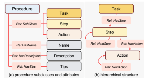
Figure 2: Overview of procedural graph structure. (a) Procedure subclass and their attribute relationships. (b) The hierarchical structure between different procedures.
