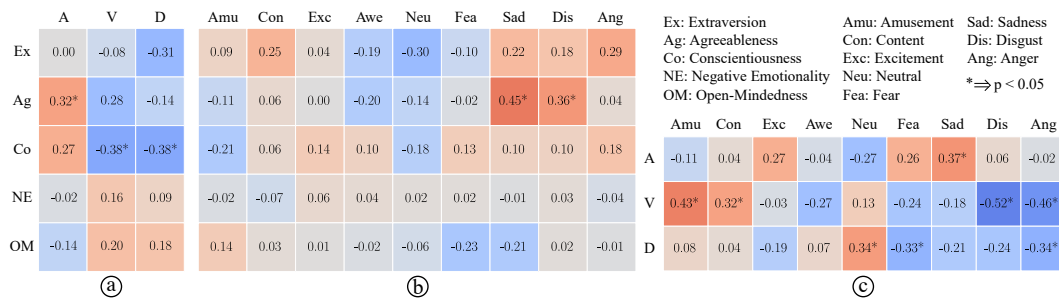
Figure 4: Pearson correlations between self-reports. (a) continuous self-ratings and personality scores (b) discrete emotions and personality scores (c) discrete emotions and continuous self-ratings.
