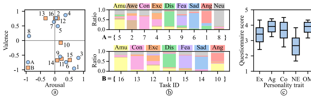
Figure 3: Participant self-reports across tasks. (a) Mean arousal-valence ratings. (b) Proportions of discrete emotions reported in Sessions A and B. (c) Boxplots of Big Five personality trait scores.
