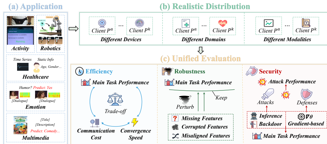
Figure 1: Framework of MARS-VFL. (a) MARS-VFL provides a diverse collection of 12 datasets from five real-world applications that align with VFL settings: human activity , robotics , healthcare , emotion , and multimedia . (b) MARS-VFL follows realistic data distributions across clients in VFL, where data from different devices , data domains , and modalities are distributed among different clients. (c) MARS-VFL offers comprehensive and unified evaluation protocols across three foundational directions: efficiency , robustness , and security , promoting future research in VFL.
