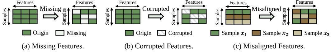
Figure 2: Illustration of Robustness. (a) Missing Features : It refers to situations where parts of sample features are missing. (b) Corrupted Features : It refers to cases where parts of sample features may be corrupted. (c) Misaligned Features : It refers to situations where features across clients are incorrectly aligned with the wrong samples.
