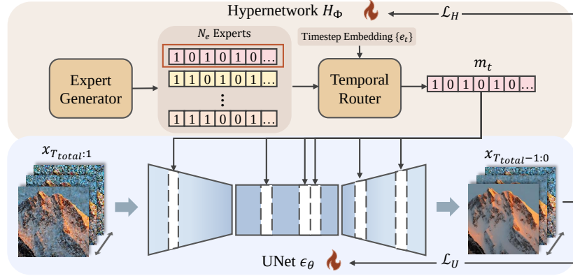
Figure 2: Overview of the ALTER framework. ALTER is a temporal-adaptive-pruning framework for diffusion models, where a hypernetwork generates layer-wise pruning configurations for expert subnetworks and assigns each denoising timestep to a corresponding expert.
