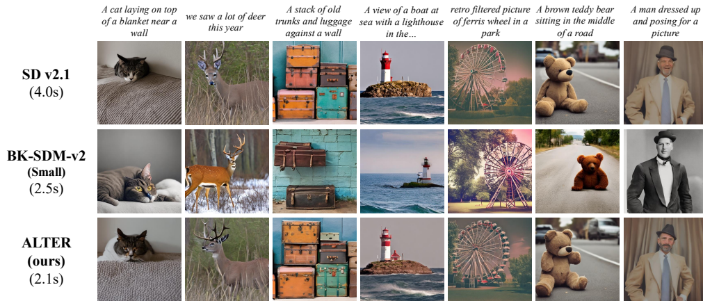
Figure 3: A qualitative comparison with original SDv2.1 and BK-SDM-Small. SDv2.1 and BK-SDM-Small adopt the 25-step PNDM while our method adopts the 20-step inference.
