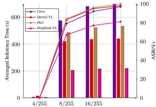
Figure 4: Average inference time (s) and ASR (%) of VMA for Sponge Examples attack across four VLMs.
