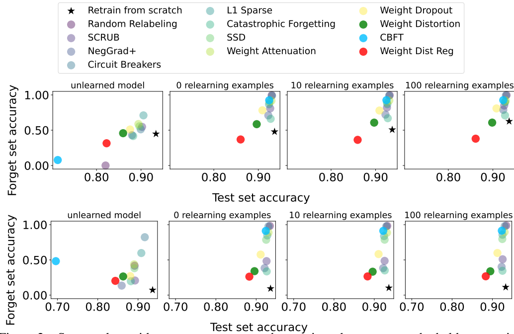
Figure 2: Scatter-plots with test-set accuracy on the x-axis and accuracy on the held-out portion of the forget set, \mathcal{D}_{F_{ho}} , on the y-axis. The left-most subplot indicates performance immediately following unlearning. The next three subplots are following a relearning attack with instances of the retain set, \mathcal{D}_R and a varying number of instances of the forget set, \mathcal{D}_{F_{re}} (0, 10, and 100, respectively). Each point is the average performance of the last 50 steps (see Fig. 11 for the whole trajectory for sub-class unlearning and Fig. 12 for the trajectory for class-agnostic unlearning). The forget set is comprised of atypical examples (from the ‘airplane’ class, i.e., sub-class unlearning for the top row and all classes, i.e., class-agnostic unlearning in the bottom row) in CIFAR-10. The figure indicates that many methods achieve near-perfect recovery of unlearned knowledge with only a small amount of model fine-tuning, even with 0 relearning examples (fine-tuning on only the retain set). Weight Distortion, CBFT, and Weight Dist Reg are introduced in Section 6.
