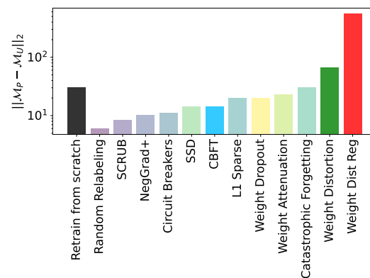
Figure 5: L_2 norm of the difference between the parameters of the pretrained and the unlearned models induced by different unlearning methods. We consider only the difference in the parameters, while ignoring the batch-norm statistics for ResNet-18 trained on CIFAR-10, where the forget set is comprised of atypical examples.
