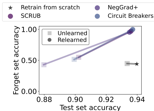
Figure 1: Fine-tuning an unlearned model on just the retain set recovers performance on the forget set! Results on CIFAR-10 using a forget set of atypical examples from class ‘airplane’.
