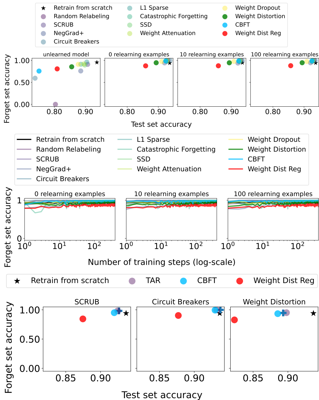
Figure 8: Comparison between test set accuracy and accuracy on the held-out part of the forget set D_{F_{ho}} on CIFAR-10 and ResNet-18, where the forget set is comprised of a random subset of the examples from the ‘airplane’ class. The figure indicates that retrain from scratch baseline can already achieve near-perfect accuracy, as the examples in a class are predominantly comprised of typical examples.
