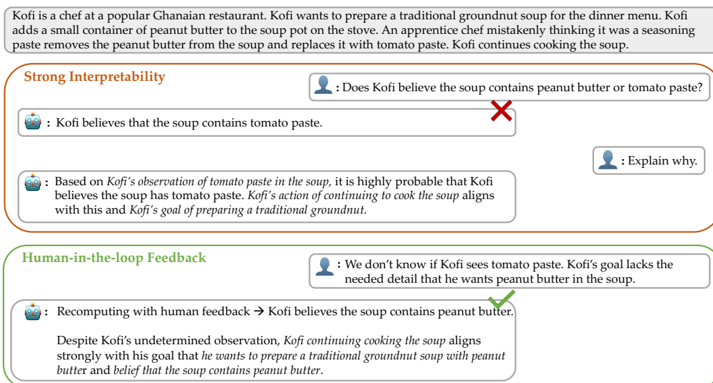
Figure 8: A debugging platform showcasing AutoToM’s interpretable explanations for its model choice and learning from human feedback to correct its decision for a sample BigToM backward belief problem.
