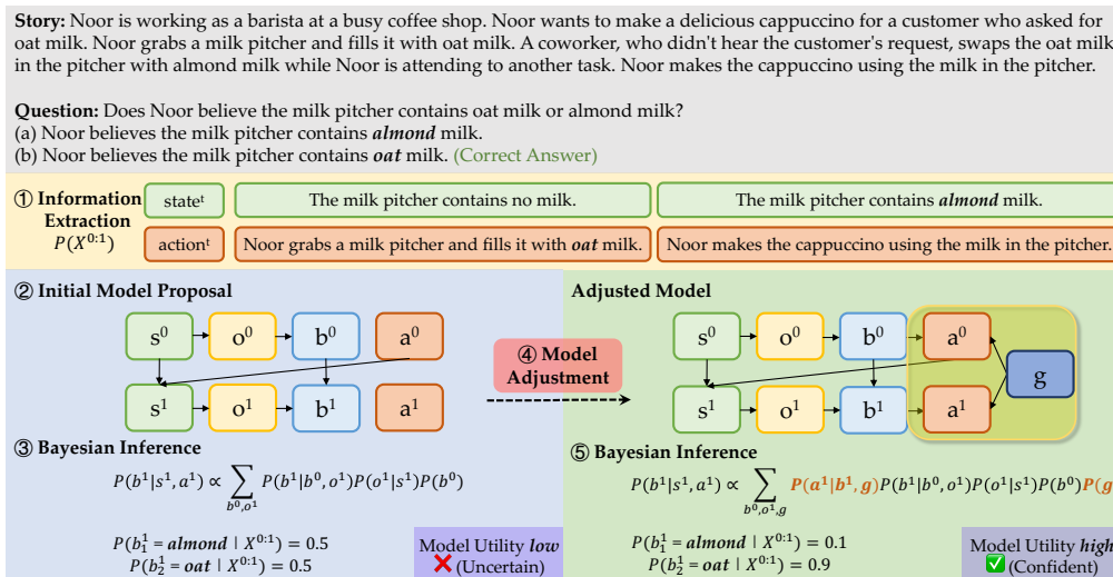
Figure 5: A qualitative example of AutoToM 's model adjustment and inference process in a false-belief scenario from BigToM [11]. We show the results from each key model step. It demonstrates how AutoToM adjusts the agent model to increase inference confidence. Detailed procedures of Bayesian inference for both the proposed and adjusted models are provided in Appendix C.5.
