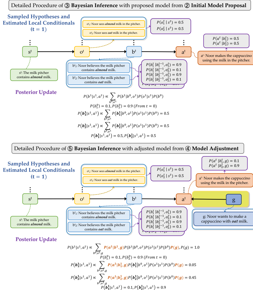
Figure 9: Detailed procedures of how Bayesian inferences are conducted for the proposed and adjusted models in Figure 5. In the initially proposed model, the belief inference results in uncertainty due to ambiguous observations. In the adjusted model, where the agent's goal is explicitly modeled, the use of goal-conditioned action likelihood P(a^t | b^t, g) instead of P(a^t | b^t) enables more accurate estimation of action likelihoods and leads to improved belief inference with high certainty.
