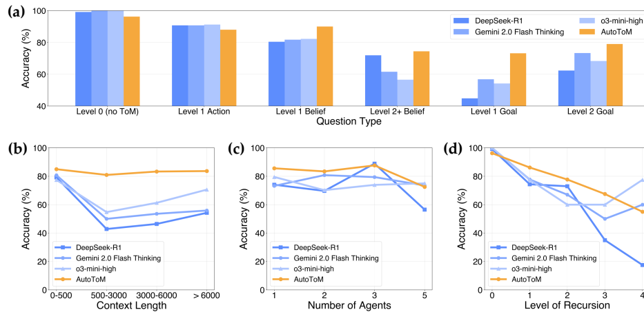
Figure 4: Comparison of AutoToM and large reasoning models across various conditions (summarized among all benchmarks): (a) question types, (b) context length, (c) the number of agents, and (d) the level of recursion. Note that “Level 1 Action” refers to Forward Action inference in BigToM, and “Level 2 Goal” refers to the Belief of Goal inference in MuMA-ToM.
