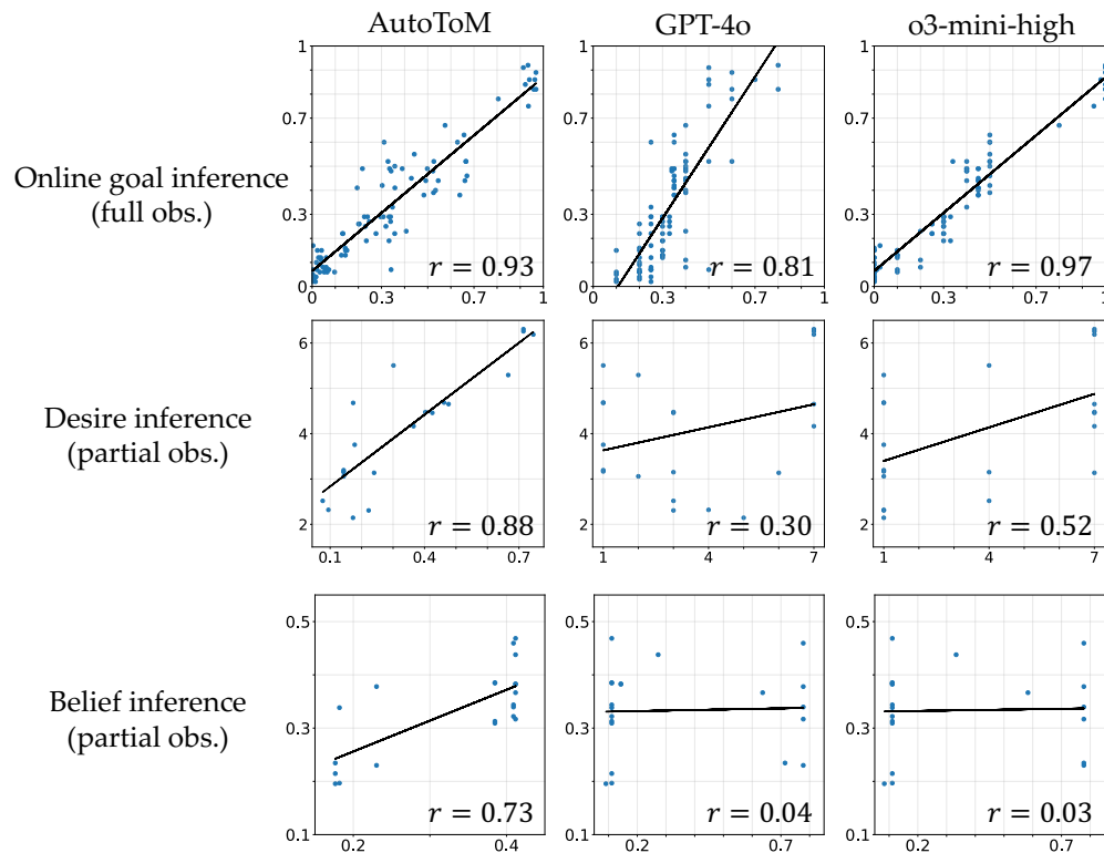
Figure 10: Comparing model and mean human mental state inferences.
