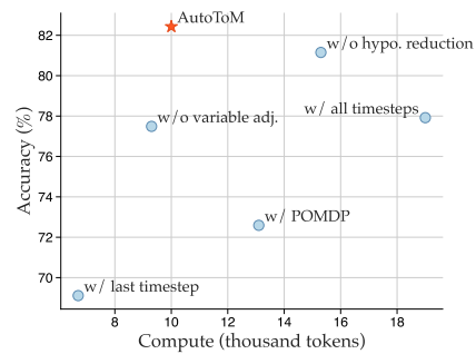
Figure 6: Averaged performance and compute of AutoToM (star) and its variants (circles) on all benchmarks.
