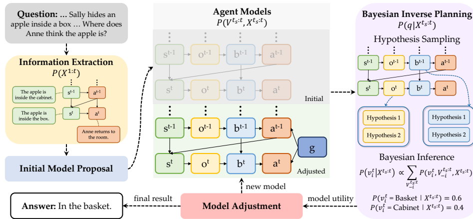
Figure 1: An overview of AutoToM . X^{t_s:t} are observable variables, V^{t_s:t} are latent mental variables, and q is the query (in this case, a mental variable v_i^t \in V^t ). t_s : t denotes timesteps from t_s to t in the context that are considered for inference. Variables s^t , o^t , b^t , a^t , g^t represent state, observation, belief, action, and goal, respectively, with solid arrows indicating dependencies defined in the models. Given a question, we extract the observable variables (information extraction) and propose an initial agent model. This is followed by automated Bayesian inverse planning and iterative model adjustment. When the model utility is high enough, we will produce the final answer based on the inference result.
