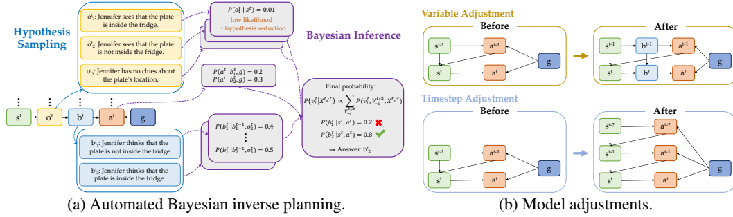
Figure 3: (a) Given an agent model, AutoToM samples hypotheses for each latent variable ( o^t and b^t in this example), remove spurious hypotheses, and conduct Bayesian inference based on estimated local conditionals. (b) Given any ToM inference problem, AutoToM refines the agent model by alternating between variable adjustment (introducing belief in this example) and timestep adjustment.
