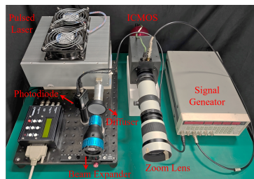
Figure 8: System Prototype.
