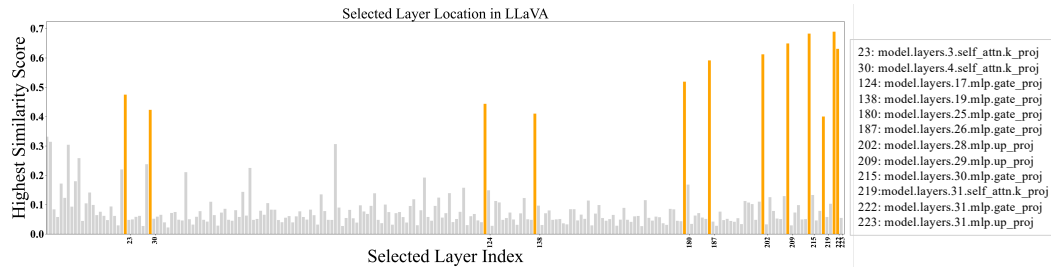
Figure 5: Selected layers in the LLaVA model for merging.
