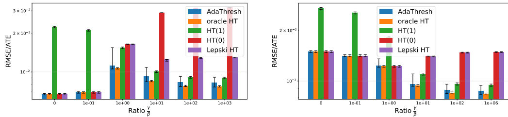
Figure 3: RMSE (normalized by the ATE) of different Horvitz-Thompson estimators for the SBM graph in Figure 2 (left panel). Left: unit-level Ber(0.5) randomization. Right: cluster-level Ber(0.5) randomization with ground truth clusters. The error bars are the empirical 95% confidence intervals around the mean.
