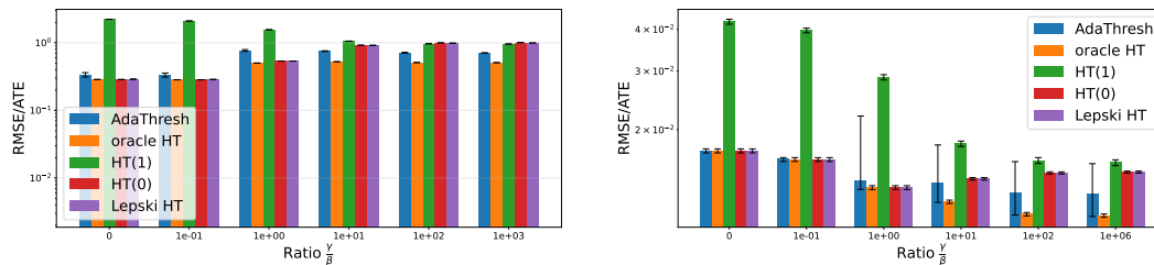
Figure 4: RMSE (normalized by the ATE) of different Horvitz-Thompson estimators for the village network in Figure 2 (right panel). Left: unit-level Ber(0.5) randomization. Right: cluster-level Ber(0.5) randomization with \epsilon(=1) -net clustering. The error bars are the empirical 95% confidence intervals around the mean.
