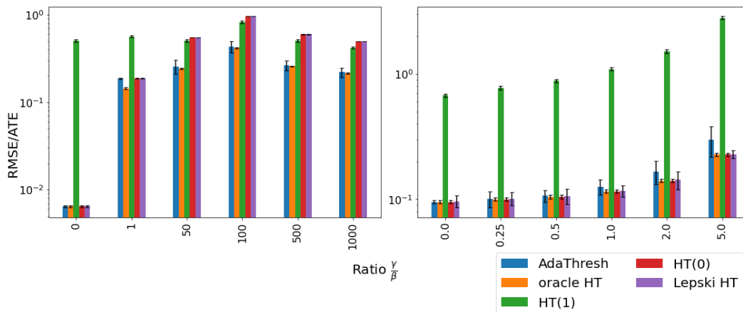
Figure 13: RMSE (normalized by the ATE) under the linear model with \psi(z_i, e_i) = g(z_i) + f(e_i) , \alpha_i = 10 , g(z_i) = \beta z_i = 10z_i , and fixed \epsilon_i generated from \mathcal{N}(0, 1) , induced by the different (local) Horvitz-Thompson estimators. Left: 2nd-power cycle graph under unit-level Ber(0.5) randomization under sigmoid f(e_i) = \gamma/(1 + \exp(-e_i)) . Right: 2nd-power cycle graph under unit-level Ber(0.5) randomization with f(e_i) = \gamma(1 - \sin(\pi \cdot e_i)) being a sine function. We focus on varying the ratio \gamma/\beta as we consider a fixed graph, with n = 1000 . The error bars are two times the standard deviation.
