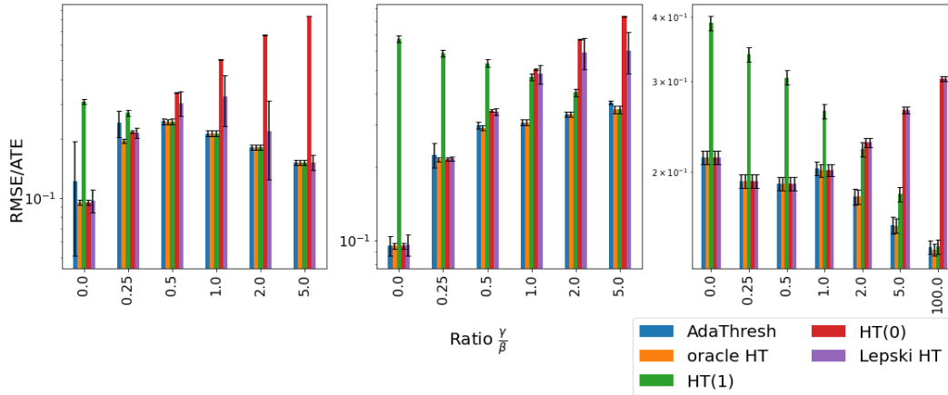
Figure 11: RMSE (normalized by the ATE) under the linear model with \psi(z_i, e_i) = g(z_i) + f(e_i) , \alpha_i = 10 , g(z_i) = \beta z_i = 10z_i , f(e_i) = \gamma e_i , and fixed \epsilon_i generated from \mathcal{N}(0, 1) , induced by the different (local) Horvitz-Thompson estimators. We focus on varying the ratio \gamma/\beta as we consider a fixed graph, with n = 1000 . Left: Cycle graph under unit-level Ber(0.5) randomization. Center: 2nd-power cycle graph under unit-level Ber(0.5) randomization. Right: 2nd-power cycle graph under cluster-level Ber(0.5) randomization with cluster sizes 5 ( =2k + 1 ). The error bars are two times the standard deviation.
