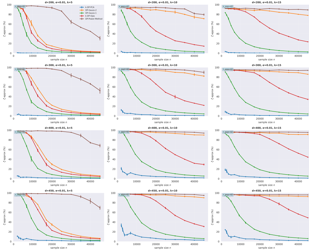
Figure 3: Comparison of k -DP-PCA and k -DP-Ojas for varying k and d (also including DP-Gauss-1 (input perturbation), DP-Gauss-2 (object perturbation), and DP-Power-Method) on the spiked covariance model. We plot the mean over 50 trials, with the bars representing the standard deviation.
