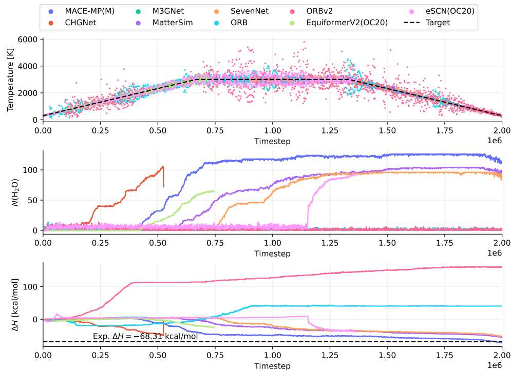
Figure S3: Hydrogen combustion via annealing NVT MD simulation ( 128 \text{ H}_2 + 64 \text{ O}_2 \longrightarrow 128 \text{ H}_2\text{O} ). Applied temperature schedule is illustrated in the top panel. The experimental reaction enthalpy of -68.31 \text{ kcal/mol} is annotated in the bottom panel [60]. CHGNet, EquiformerV2(OC20), eSCN(OC2), and M3GNet could not finish 1 ns MD trajectories. Experimental adiabatic flame temperature of hydrogen ranges from 2380 K (air) to 3000 K (pure \text{O}_2 ) [61]. Only MACE-MP(M) and EquiformerV2(OC20) ignite within this region. Runtime performance and center-of-mass drift are available in Figure S4.
