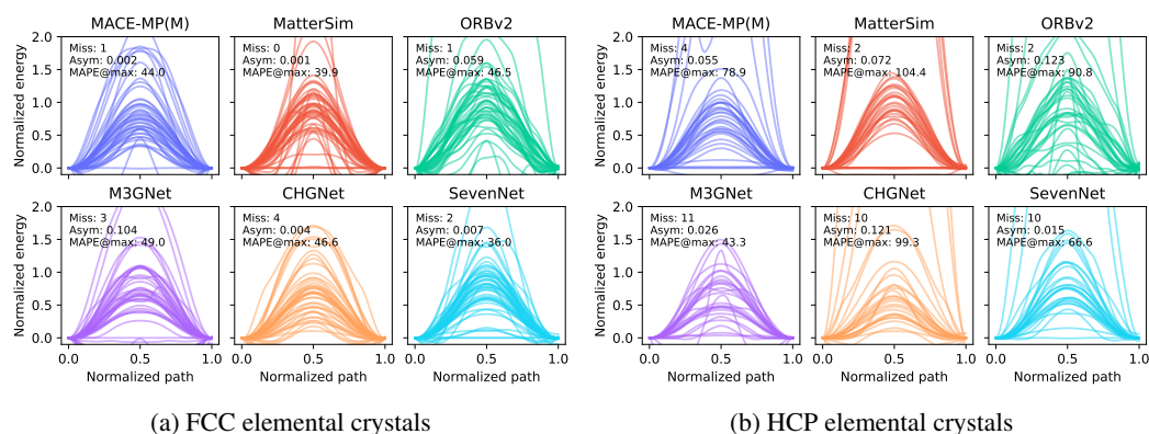
Figure 5: NEB profiles of vacancy migration in FCC (a) and HCP (b) elemental crystals. All path lengths are normalized to 1, and all energies are normalized by PBE vacancy migration energy barrier E_{\text{vm}}^{\text{PBE}} as given in [31]. Number of missing predictions, average path asymmetry, and MAPE of maximum energy barrier are annotated on top left.
