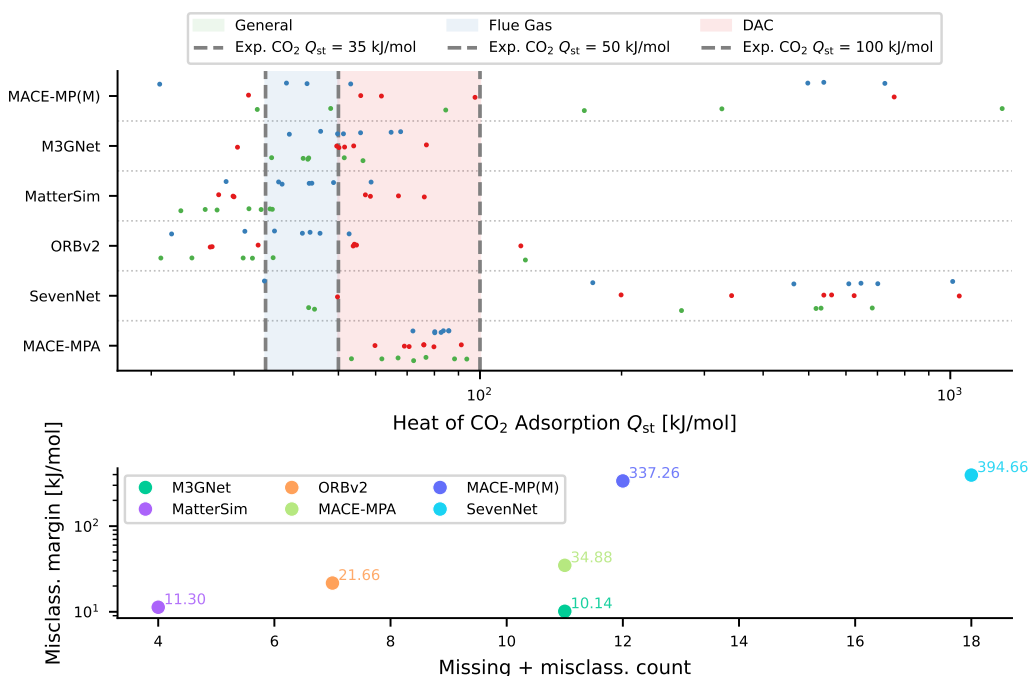
Figure S8: Classification of MOFs based on predicted heat of CO 2 adsorption. (Top) Three classes of MOFs based on experimental CO 2 Q_{\text{st}} measurements: (1) general (green area and points), (2) flue gas (blue area and blue points), and (3) DAC (red area and points). The perfect classifiers should predict Q_{\text{st}} of CO 2 in the corresponding regions. (Bottom) Mean misclassification margin and count of misclassified and missing MOFs.
