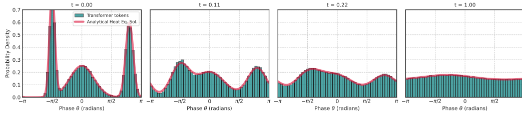
Figure 3: Evolution of the tokens distribution in the forward scenario for the second phase in \mathbb{S}^1 .
