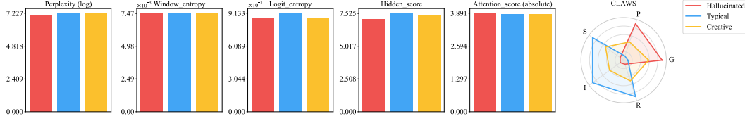
Figure 4: Visualization of class-wise average scores for each method, computed on the reference set generated using Qwen2.5-math-7B-inst. To enhance visual clarity, the normalization range is clipped between 0.1 and 0.9 for CLAWS. Visualizations for all models are presented in Figure 9.
