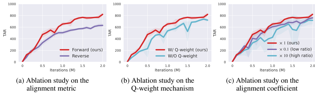
Figure 3: Ablation study curves. We select the Dog-run task (223/38 state/action dims) in DMC Suite with the highest dimensionality to perform all ablation experiments.
