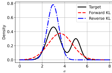
Figure 13: Comparison of forward KL and reverse KL on a fitting task. This example highlights a key issue: when the planner is multimodal but the policy is unimodal, reverse KL may fail to sufficiently cover high-density regions of the target distribution , still resulting in significant mismatch and poor performance. In contrast, forward KL provides a more stable alignment strategy , promoting broader coverage of the target distribution and preventing premature collapse.
