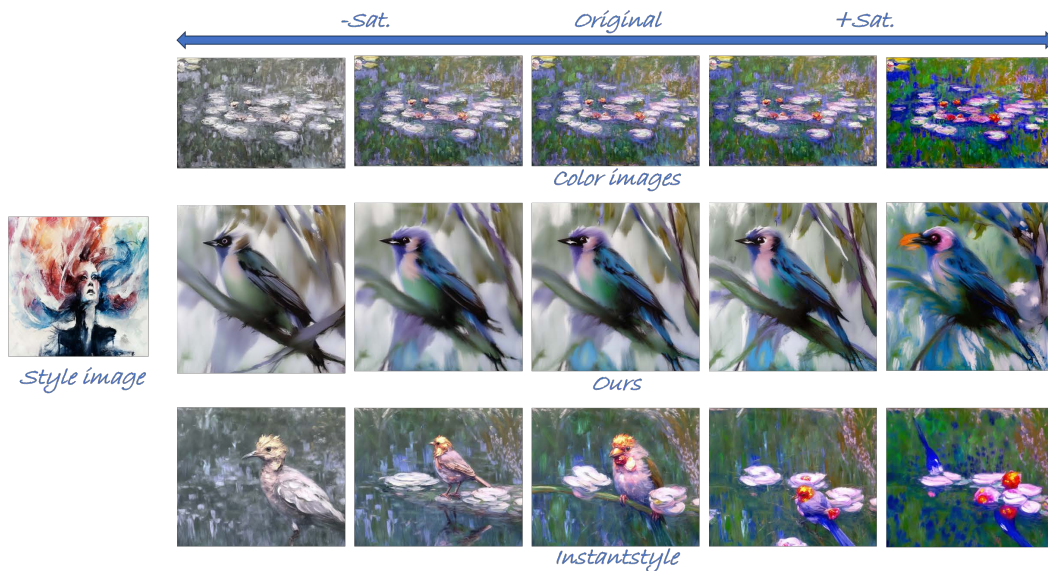
Figure 21: Compared to InstantStyle, SADis preserves the content more effectively under saturation variations.
