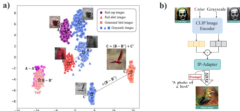
Figure 4: a) Image-prompt additivity : Image encoder latent space enables color extraction via grayscale subtraction. This color information can then be added to latent representations of other grayscale images; b) By subtracting the grayscale image embeddings from the color image embeddings, we can effectively remove the texture information and isolate the color information.
