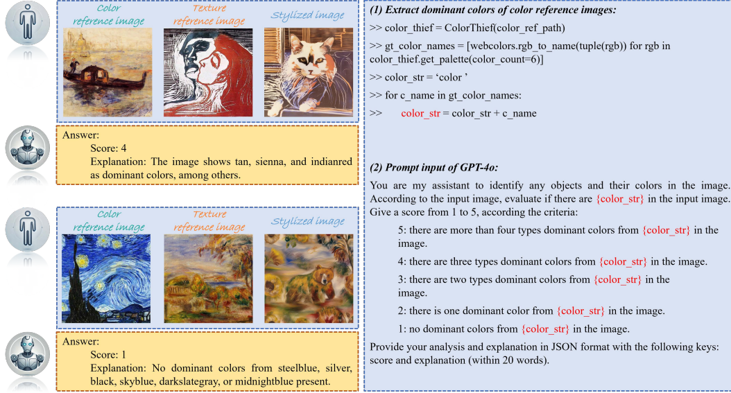
Figure 12: GPT-4o metric for color alignment evaluation.
