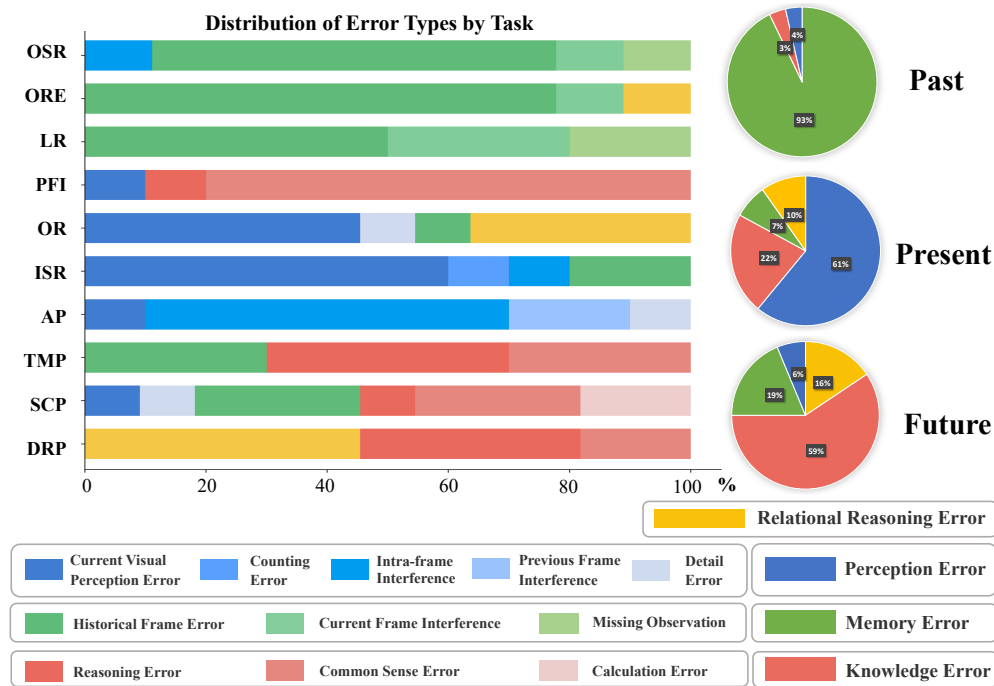
Figure 6: Quantitative error analysis by type for choice-based questions in EOC-Bench.
