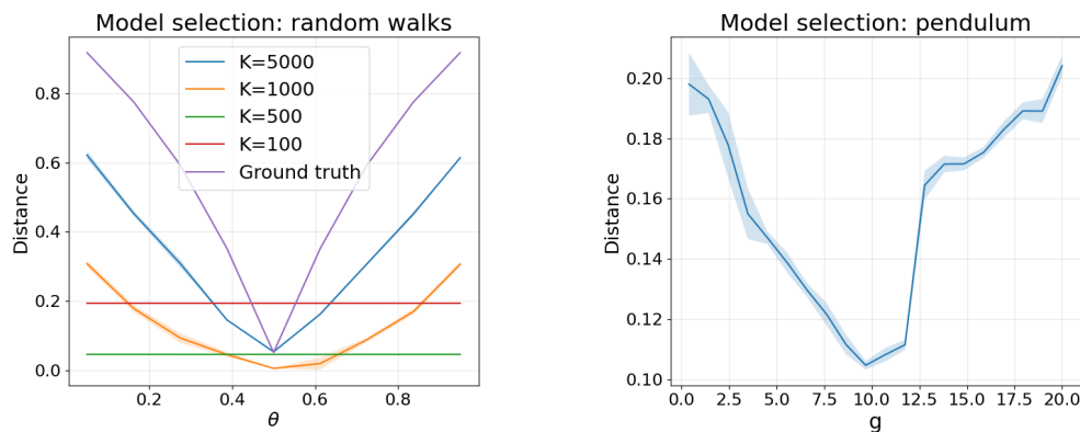
(a) Distances between the true dynamics ( \theta = 0.5 ) and the different models in the model class, for different values of the parameter \theta and the number of iterations K . (b) Distances between the true dynamics ( g = 9.8 ) and the different models in the model class, for different values of the gravity parameter g .
