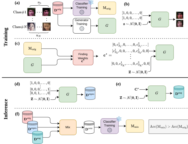
Figure 3: Overview diagram of AugGen: (a) A labeled dataset, D^{\text{orig}} , is used to train a class-conditional generator, G(\mathbf{Z}, c) , and a discriminative model, M_{\text{orig}} . (b,d) Reproduced dataset, D^{\text{repro}} , closely mimics D^{\text{orig}} under the original conditions. (c) We find new condition vectors, C^* , to generate an augmented dataset, D^{\text{aug}} , using the generator. (f) Augmenting D^{\text{orig}} with D^{\text{aug}} boosts M_{\text{orig}} performance without auxiliary datasets or models.
