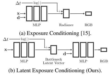
Figure 5: Exposure Conditioning. While prior works [15] condition the color prediction on the log exposure by adding it onto the radiance (5a), we also perform the log transformation but condition in latent space instead (5b), leading to improved performance and more stable optimization.
