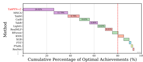
Figure 2: Probability of Achieving the Maximum Accuracy or Minimum RMSE across 273 datasets. Values inside rectangles show the percentage of datasets on which a method achieves the best result.
