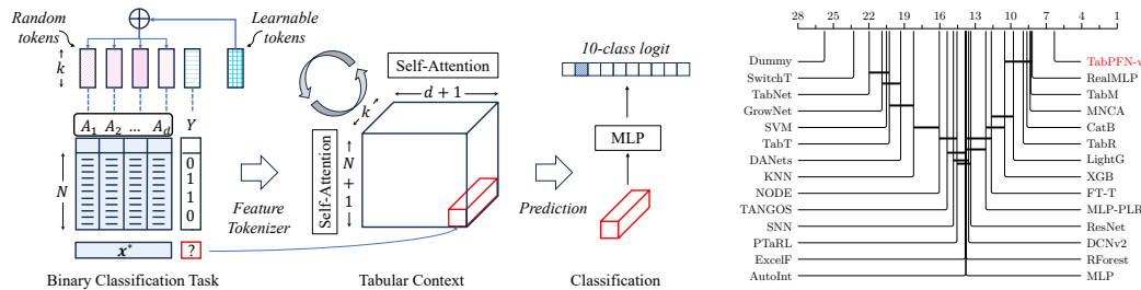
Figure 1: Left: Illustration of TabPFN v2’s mechanism for binary classification [28]. \{A_1, \dots, A_d\} denote d attributes of the task. Training examples and a test instance are combined into a tabular context and transformed into a (N + 1) \times (d + 1) \times k tensor using a combination of learnable and randomized tokens. Two types of self-attention are applied alternately across rows (inter-sample) and columns (inter-feature). The output token corresponding to the (dummy) label of the test instance is processed through an MLP to generate a 10-class logit. Right: Wilcoxon-Holm test at a significance level of 0.05 over 273 small- to medium-scale datasets. We omit the 27 datasets used to select TabPFN v2’s checkpoint from the 300 datasets in [75].
