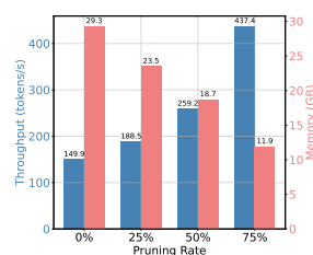
Figure 3: Memory footprint and inference speed of pruned Qwen1.5-MoE-A2.7B.
