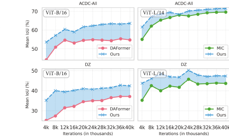
Figure 4: Convergence curve comparison.
