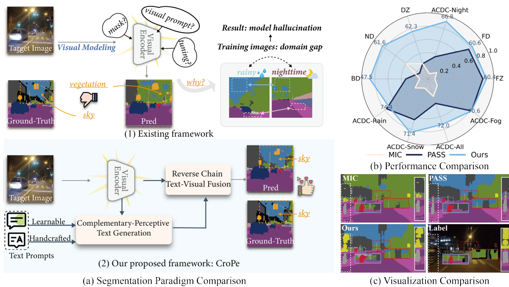
Figure 1: Comparison between our CroPe and existing methods: (a) In contrast to existing methods relying solely on visual modality, our CroPe integrates visual and text modality. (b) Our CroPe outperforms existing methods in many adverse scenarios. (c) Existing methods often produce hallucinations (e.g., incorrectly classifying the sky as trees). We highlight the differences between our CroPe and existing methods using dashed boxes, and zoom in with solid boxes for emphasis.
