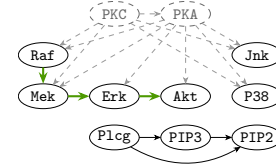
Figure 8: Sachs' graph. Green edges mark proxy-identifiable effects.
