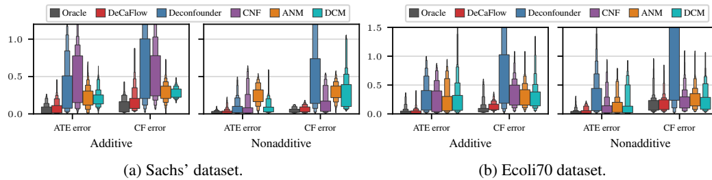
Figure 7: ATE and CF error boxenplots [23] of different CGMs on the (a) Sachs and (b) Ecoli70 datasets, aggregating over all identifiable direct effects (see Figs. 1 and 8) after intervening on their 25th, 50th, and 75th percentiles over 5 random initializations.
