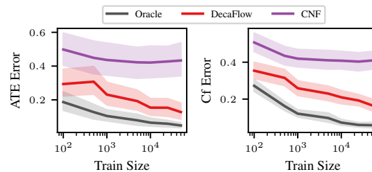
Figure B.4: ATE and Counterfactual error in Sachs' additive dataset, varying the number of train samples. Test size are the same for all realizations. Metrics and 95% CI over 10 realizations and all confounded identifiable effects, intervening in percentiles 25 and 75 of each intervened variable. Oracle represents a CNF that observes the confounders.
