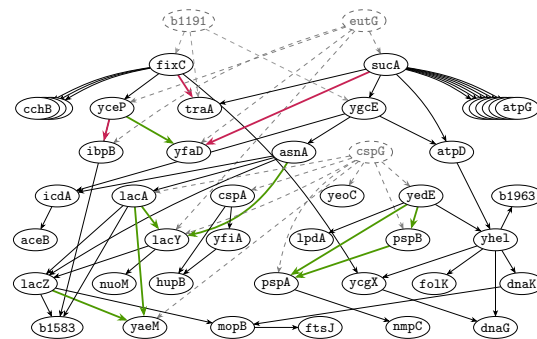
Figure 1: DeCaFlow can be effortlessly applied to highly complex causal graphs , as that of the Ecoli70 dataset [66], with multiple hidden confounders and dozens of variables. We dash hidden confounders, and highlight direct hidden-confounded effects as identifiable (and thus correctly estimated by DeCaFlow ), or unidentifiable .
