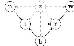
Figure A.2: Example for which Prop. A.2 applies, and where \mathbf{b} \neq \emptyset .
