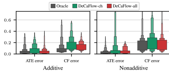
Figure B.3: Ablation for posterior factorization in Ecoli70 dataset. Boxenplots of error metrics in the identifiable edges of Fig. 1. DeCaFlow-ch uses Eq. 57 and DeCaFlow-all uses Eq. 60 for posterior factorization.
