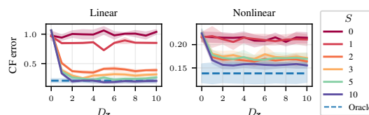
Figure 6: CF error as we increase the number of proxies, S , and the latent dimensionality, D_{\mathbf{z}} . Plots show mean and 95 % CI over 5 realizations, intervening on the 25th, 50th, and 75th percentiles of t .
