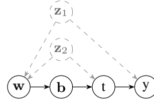
Figure A.5: Napkin causal graph [53].
