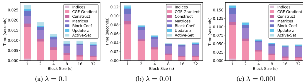
Figure 4: ECCD Time Decomposition Plot (Duke)
