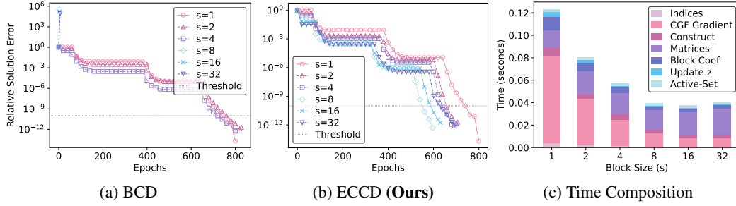
Figure 2: Results on the duke dataset with \alpha = 0.5 and \epsilon = 0.01 . (a) Convergence of BCD exhibits numerical instability as block size s increases. (b) Convergence of ECCD remains stable even for s = 32 . The convergence threshold is set to 1e-10 . (c) Breakdown of ECCD's runtime components.
