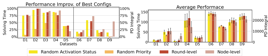
Figure 5: Left: Performance improvement of the best configurations found by different random strategies on nine benchmarks. The y-axis represents the relative improvement compared to the default setting. Right: Average performance of configurations sampled by different random strategies on nine benchmarks. The y-axis represents the real performance under two metrics. Specifically, Datasets D1–D5 use solving time (left) as the metric, while D6–D9 use PD integral (right). Each bar represents a specific strategy to get random configurations.
