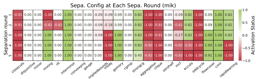
Figure 11: Separator configs at each separation round for MIK benchmark.
