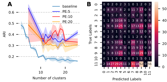
Figure 18: A ARI between models seeds for models trained on all 1244 neurons. B Confusion matrix between predictions of the model trained on 1000 neurons and labels suggested in Willeke et al. [51]
