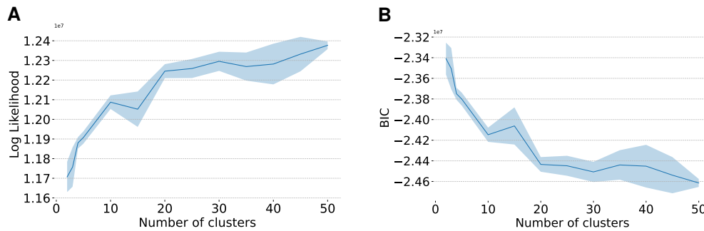
Figure 19: A : Log likelihood estimation. B : Calculation of BIC.
