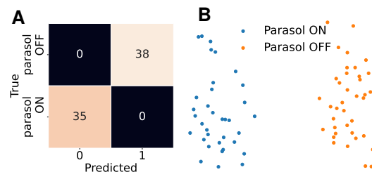
Figure 9: A: DECEMBER predictions. Pretraining length: 20 epochs. Same predictions for GMM and k-means. All methods have ARI 1. B: t-SNE projections of the corresponding cells.
