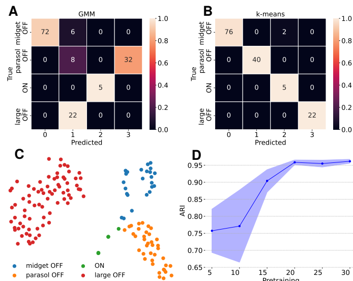
Figure 10: All plots show evaluations of seed 4 of the trained marmoset RGC model [15] for retina 1 used in the main part of this paper. A: GMM predictions. B: k-means. C: t -SNE projections of the corresponding cells. D: ARI for different length of pretraining. Longer pretraining seems to be beneficial with ARI stabilizing after pretraining of 20 epochs.
