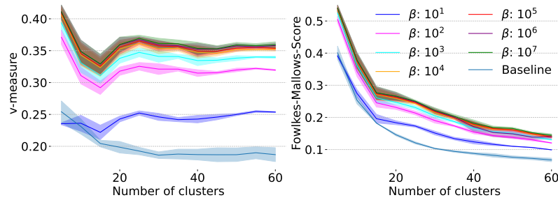
Figure 14: V-measure and Fowlkes-Mallows-score for PE 10, 15 clusters.
