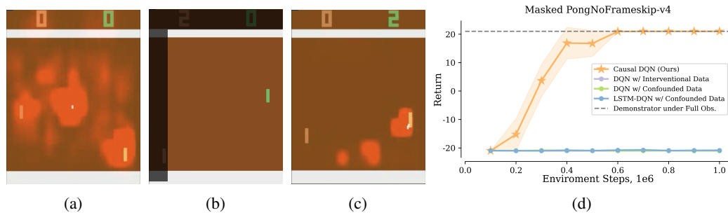
Figure 2: (a) A saliency map of the behavioral policy in Pong that tracks the opponent's location and score board; (b) a confounded Pong game where the opponent's location and score board is masked; (c) a saliency map of the conservative policy focusing on only itself and the ball; (d) the average return of our causal DQN and the standard DQN baselines. Baseline curves are overlapped.
