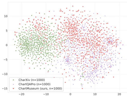
Figure 5: We show a t-SNE visualization, comparing CLIP encodings [31] from 1000 randomly sampled charts in CHARTMUSEUM against those from several real-image based chart benchmarks.
