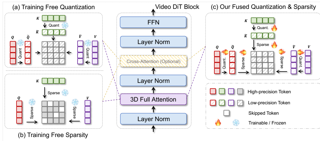
Figure 1: Comparing previous training-free quantization (a) and training-free sparsity (b) approaches reveals substantial accuracy degradation and a lack of compatibility when used independently. In contrast, our FPSAttention framework (c) integrates low-precision and sparse patterns in a single training process, yielding near-zero accuracy loss and seamless deployment.
