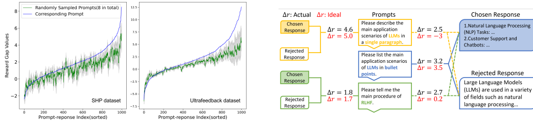
Figure 1: Left: reward gaps calculated with corresponding prompt and randomly sampled prompts using QRM-Llama3-8B 1 on two different datasets that were used for training. When calculating with other prompts, the curves show the mean and the std. Right: illustrative failure case where the reward gap overly depends on the responses. Solid lines represent corresponding prompt-response pairs (used in training), while dashed lines represent non-corresponding pairs (unseen during training). Since the reward gap overly depends on the responses, it generalizes poorly to novel prompt-response pairs constructed even with seen prompts.
