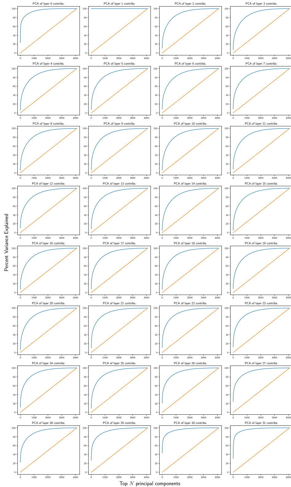
Figure A2: Percent variance explained by the top n principal components vs n , graphed on the blue line. The orange line is what we would expect if contributions were isotropic. For layers where TLM is most active (4 to 20), the first 500-800 principal components explain 80% of the variance in contributions, demonstrating that contributions are anisotropic.
