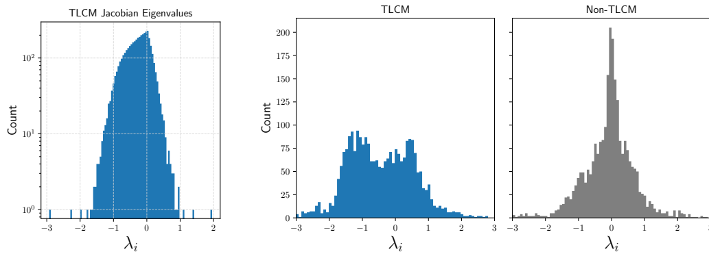
(a) Nearly 3/4 of the 4096 eigenvalues of the Jacobian \bar{J} are negative. (b) Left: Strongest components of \mathbf{a}_t are corrected or reinforced by the TLCM Jacobian. Right: For non-TLCM Jacobians, \mathbf{a}_t 's strongest components are predominantly untouched.
