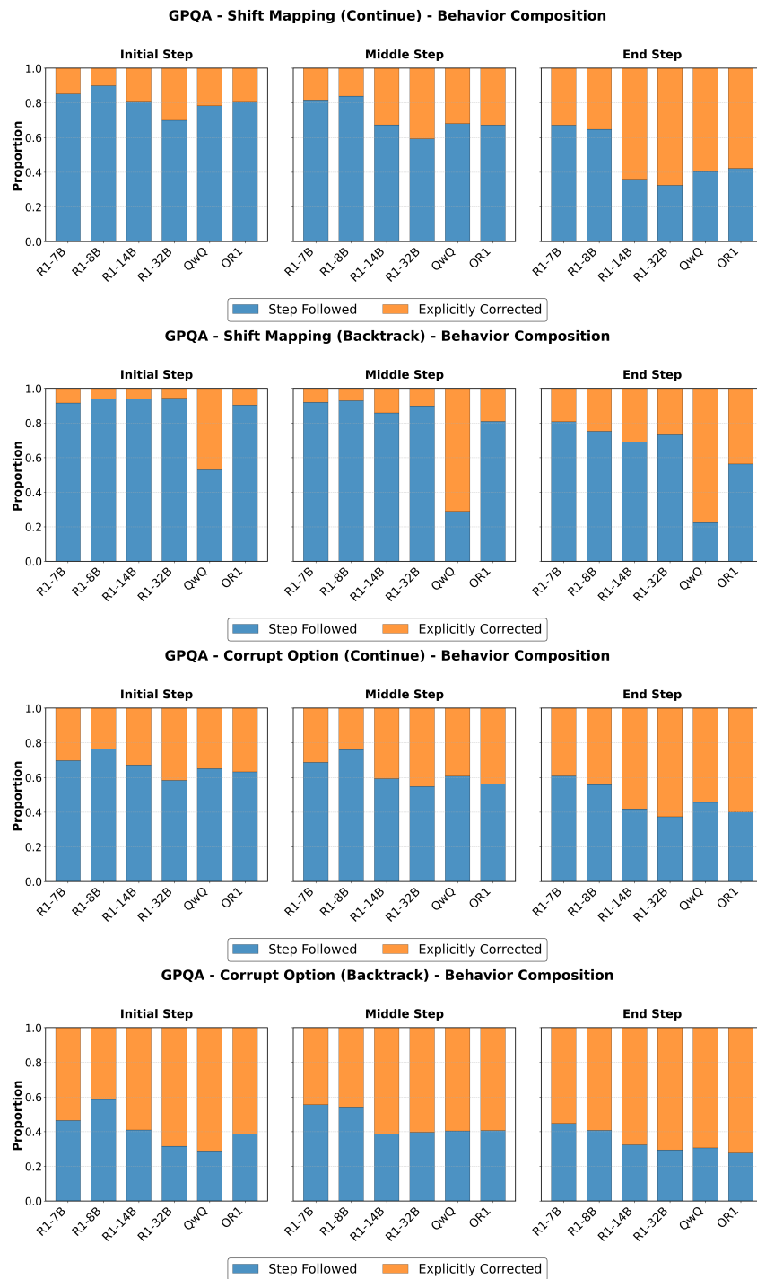
Figure 7: Different model response behaviors across four intervention setups by testing on GPQA.
