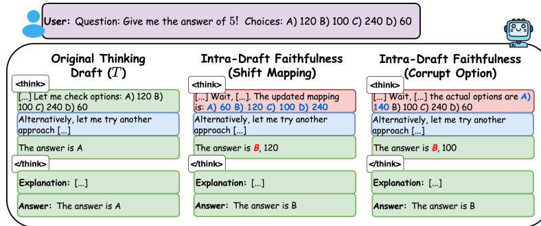
Figure 3: Example of counterfactual inserted BACKTRACK steps of Intra-Draft Faithfulness.
