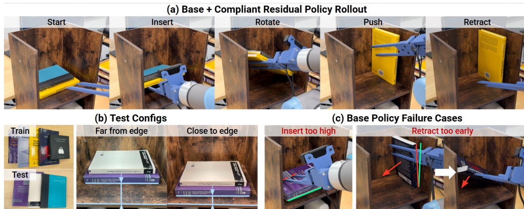
Figure 4: Book Flipping Task. (a) Policy rollout of [Compliant Residual] policy trained with [On-Policy Delta] data, demonstrating accurate insertion motions and forceful pushing strategy. (b) Different test scenarios. (c) Typical failure cases of the base policy: inserting too high above the book and missing the gap; retracting the fingers before the books can steadily stand.
