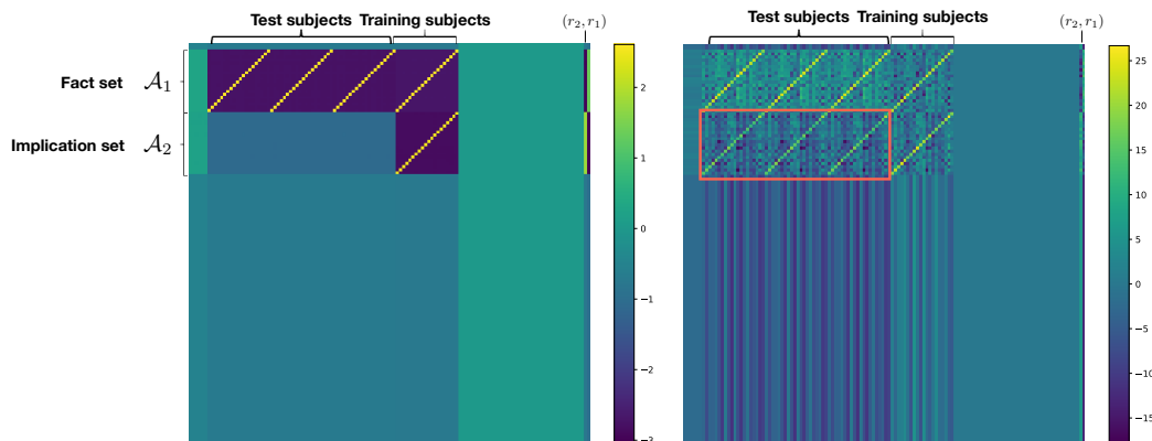
Figure 4: Comparison of full weights of trained one-layer linear attention models. Left: Non-factorized model. Right: Factorized model. The factorized model shows strong OCR capability compared to the non-factorized model.
