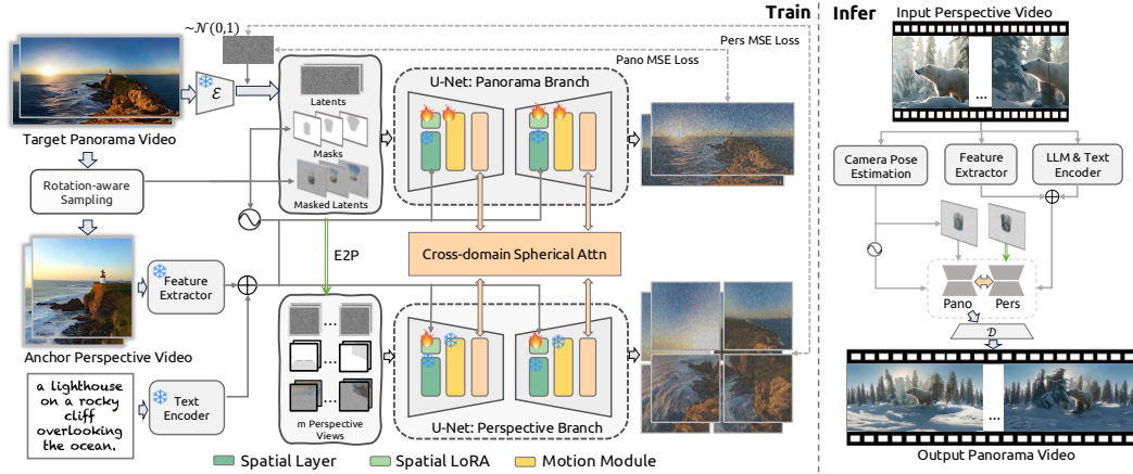
Figure 2: Pipeline of Imagine360. Given a perspective anchor video, Imagine360 uses a dual-branch denoising structure across panorama and perspective domains, featuring cross-domain spherical attention with antipodal masking for modeling long-range antipodal motion, and rotation-aware designs to handle varying camera rotations.
