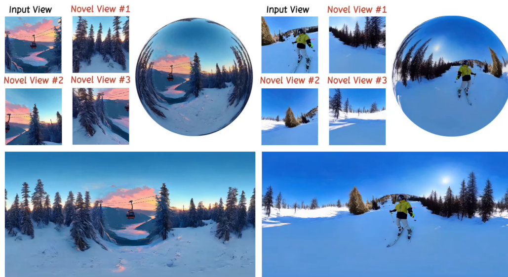
Figure 1: Overview of Imagine360. Imagine360 lifts standard perspective video into 360° video, enabling dynamic scene experience from full 360 degrees. Our approach achieves high-quality texture and plausible spherical motion patterns for both generated video (left) and in-the-wild video (right). Best viewed with Acrobat Reader for the animated 360 videos . More examples please visit our webpage .
