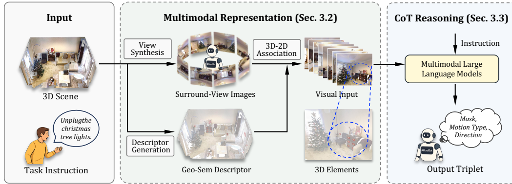
Figure 2: AffordBot Overview. Our method first constructs a holistic multimodal representation designed to bridge 3D scenes with 2D-native MLLMs. This process involves view synthesis, extraction of geometric-semantic descriptors, and their association. Then, our designed Chain-of-Thought (CoT) paradigm guides the MLLM to ultimately predict a structured triplet for the task.
