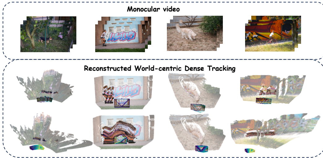
Figure 3: Qualitative results on DAVIS dataset. Our method can output both reliable camera trajectories and world centric dense tracking. The second row visualizes 3D tracking results on temporally spaced keyframes, while the third row shows complete tracks across continuous frames.
