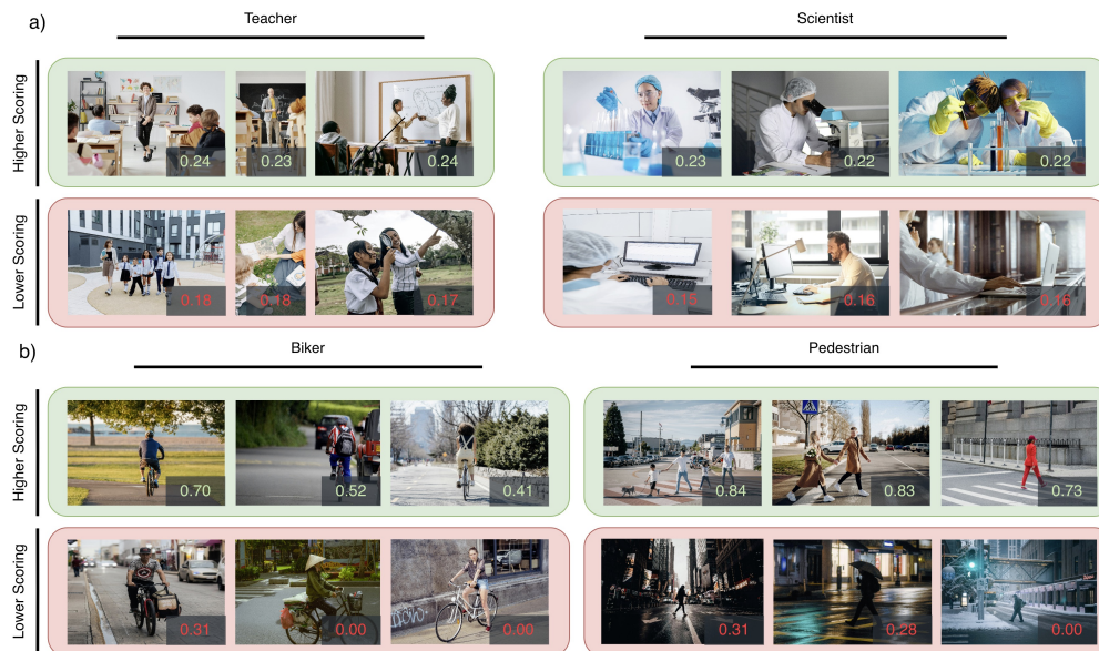
Figure 10: Real images that elicit high (green) and low (red) scores from the (a) CLIP and (b) YOLO classifiers across different object categories. Each triplet shows the top and bottom scoring examples per class for CLIP and YOLOv8.
