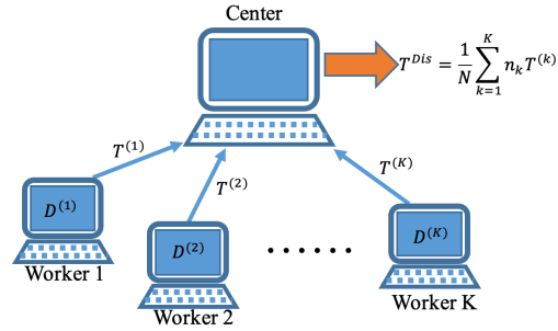
Figure 2: A distributed framework with K worker machines connected to a central processor. The k -th machine computes a local statistic T^{(k)} using its local data D^{(k)} , and then transmits it to the central processor. The central processor subsequently computes the distributed statistic T^{Dis} based on the K local statistics.
