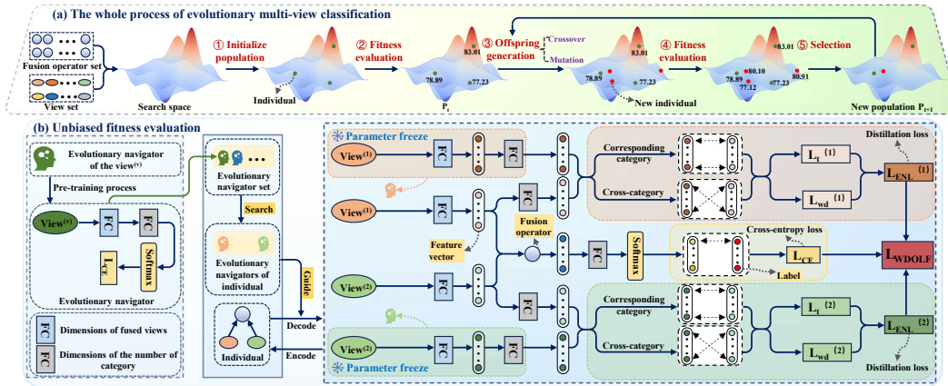
Figure 2: The overview of EFB-EMVC
