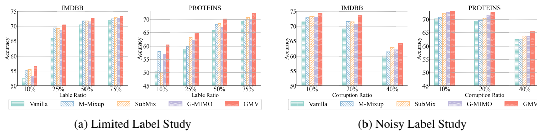
Figure 3: Comparison study between GMV and other methods for different ratio of label/varying levels of label corruption on IMDBB and PROTEINS for GCN.
