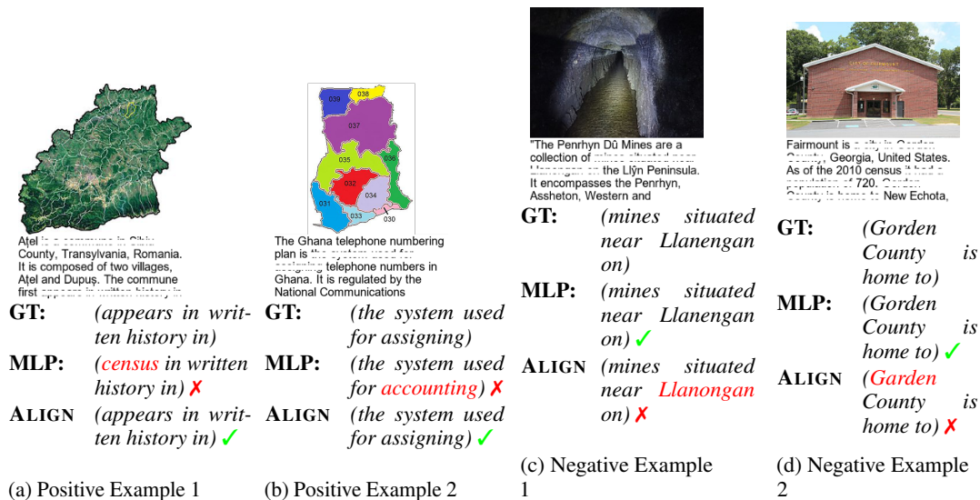
Figure 6: Case Study for Pixel-Level Tasks. We provide examples of our proposed ALIGN connector compared with a Multi-Layer Perceptron (MLP) connector. The ALIGN connector tends to better map visual elements to common words. GT is the ground truth.
