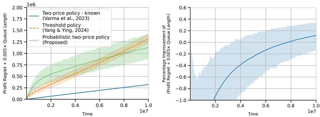
(a) \mathbb{E}[R(t)] + wt\text{AvgQLen}(t) . (b) Percentage improvement over the threshold policy [1].
