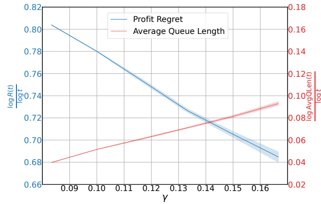
Figure 5: Tradeoff between regret and average queue length.
