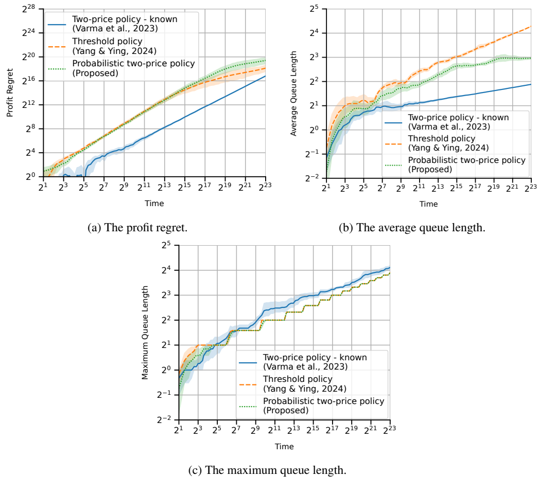
Figure 12: Comparison of regret, average queue length, and maximum queue length among the two-price policy (no learning, known demand and supply functions) [2], the threshold policy [1], and the proposed probabilistic two-price policy , in a multi-link system.
