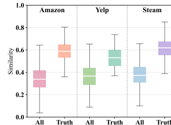
Figure 3: Item-generation task.
