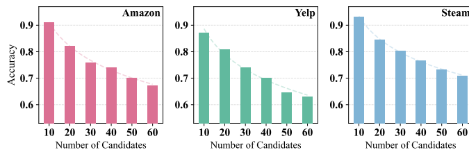
Figure 2: Item-retrieval task.
